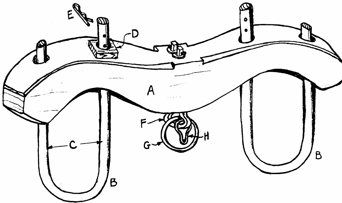
Figure 3: Parts of a traditional neck yoke: A – yoke beam; B – bows; C – bow width and size of yoke; D – spacer block; E – bow pin; F – staple; G – pole ring; H – chain hook.
