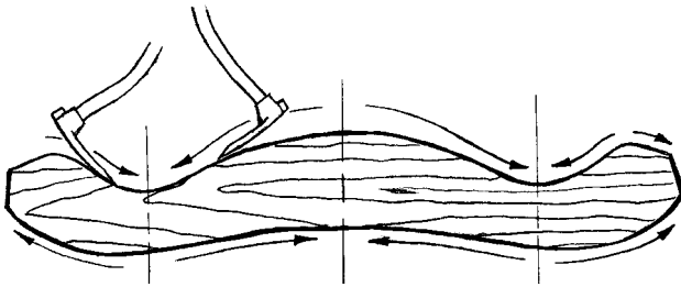
Figure 12: On a straight-grained beam, the direction of cut will move from high points to low points. Follow the arrows. If the tool is digging in or leaving a rough cut, try reversing and cutting from the opposite direction.
