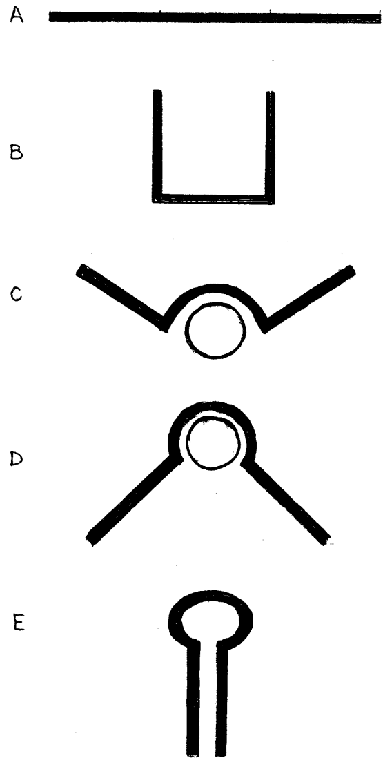
Figure 27: A staple can be formed in these steps: A-Cut bar to length, B-bend into sharp cornered U-shape over anvil corners, C & D-bend over anvil horn with pipe extensions over each end, E-adjust stems to parallel by clamping in a vise with a 1 inch spacer between.
