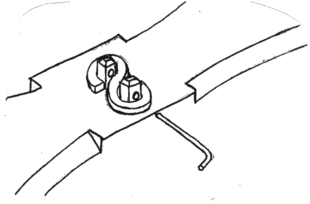
Figure 33: A pin is placed through the top of the staple and bent over the "S" washer to secure the staple.
