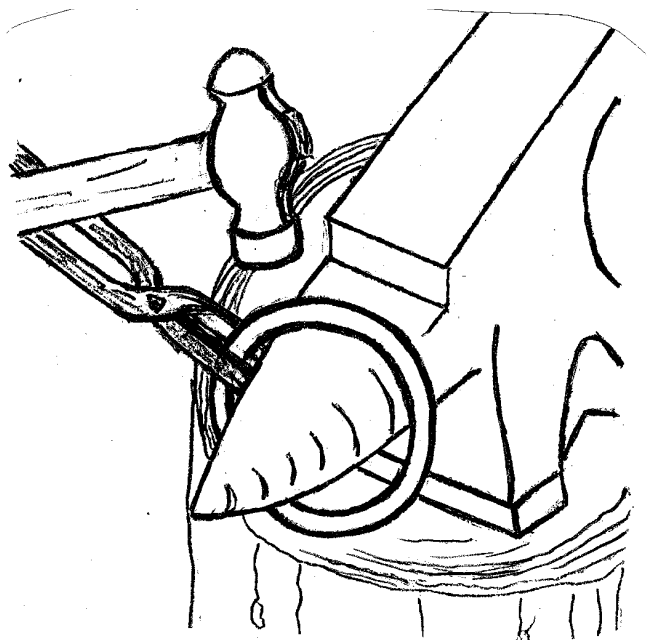
Figure 29: Finish shaping the pole ring on the horn of the anvil or on a mandrel.
