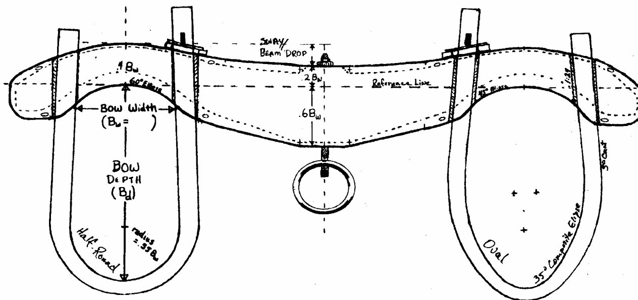
Figure 4: Tillers' Plans for a Traditional North American Neck Yoke.
