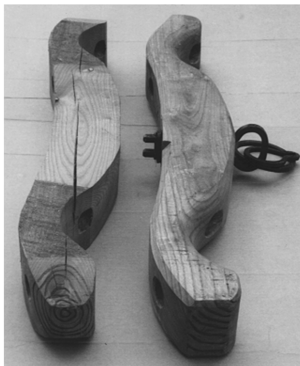
Figure 6: Two yoke beams made of sassafras wood and dried under similar conditions. The beam on the left with large cracks was made from an 8-inch diameter log. The beam on the right was made from a section of a 14-inch log. It dried without checking.
