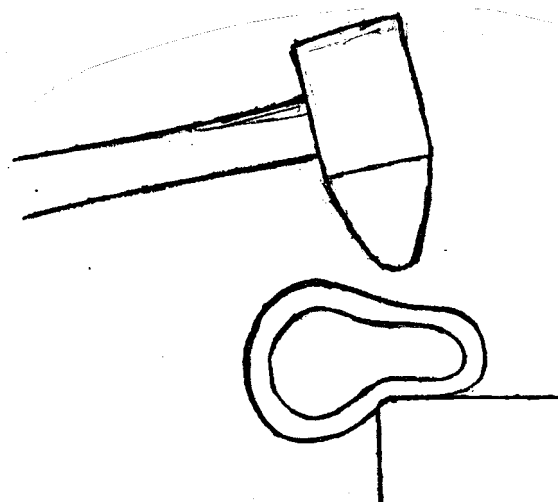
Figure 31: Form the pear shape of the grab ring on the edge of the anvil. Only heat the half of the ring that is being bent at the moment.
