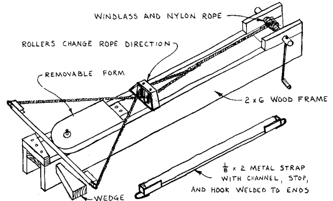
Figure 20a: Tillers bends bows on a simple jig with a windlass.
