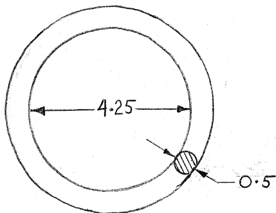
Figure 30: Calculate the length of stock from its diameter plus its thickness.
