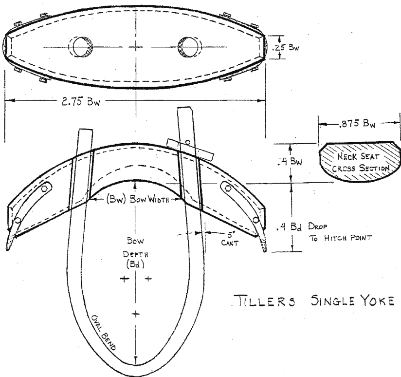
Figure 37: Tillers' Plan for making a single ox yoke.
