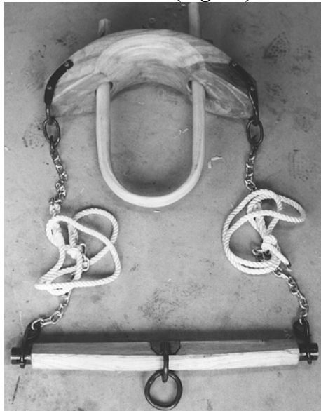
Figure 38: A single yoke laid out with rope traces to a singletree.
