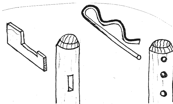
Figure 24: Wood or metal bow pins keep the bow in the yoke beam.
